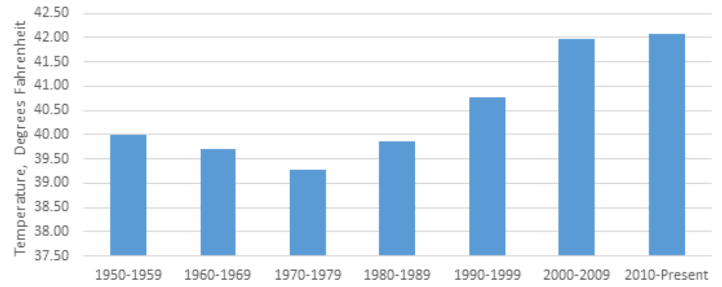
Figure 2: Mean Temperature
